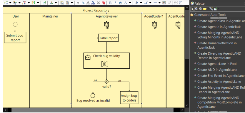
Fig. 7: Platform-independent implementation.
