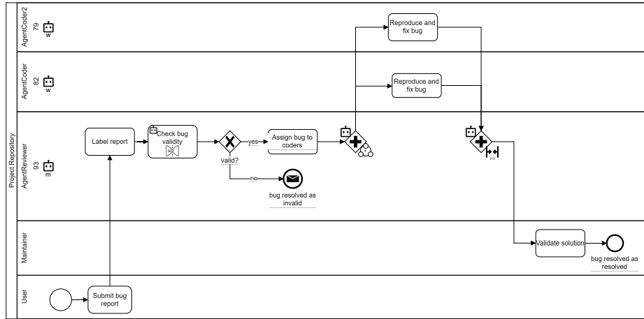
Fig. 5: Running example with our extension notation.
