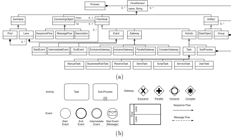
Fig. 1: Simplified (a) metamodel of BPMN and the corresponding (b) notation.
